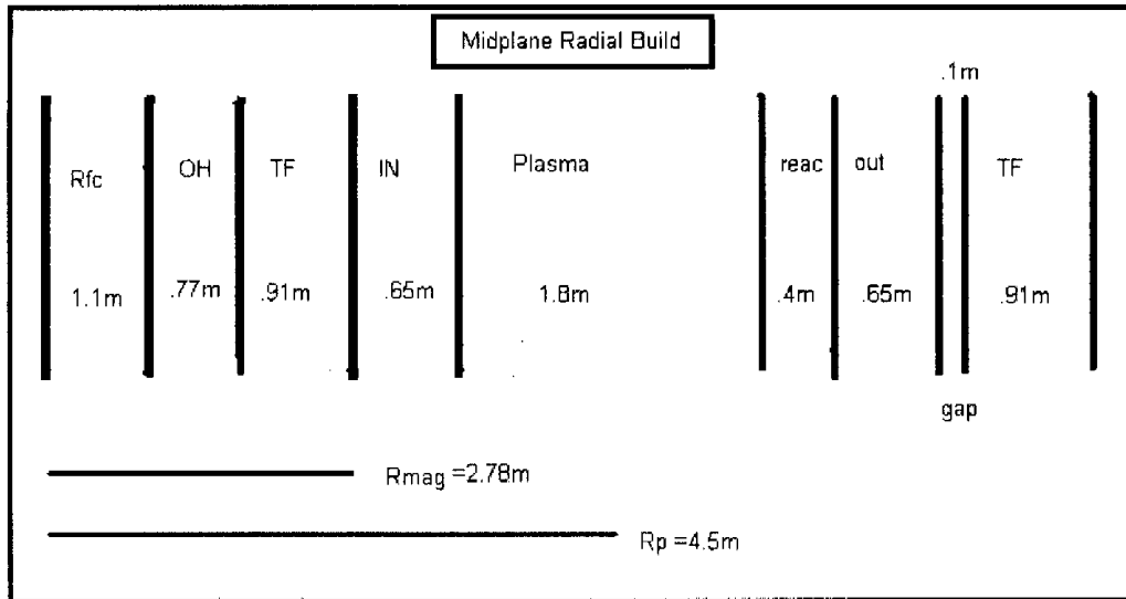
Figure 1: Radial Build of FTWR-SC (R fc = flux core, OH=OH coil, TF=Toridal Field coil, IN=Inner shield, Reac=Reactor, Out=Outer shield)
