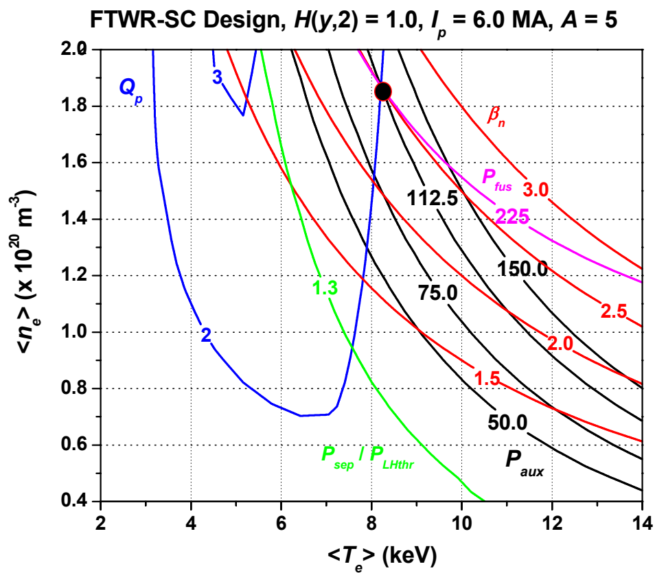
Figure 2: Plasma Operating Contour Plot ( P_{aux} is the auxiliary heating power; P_{sep}/P_{LHthr} is the ratio of the power crossing the separatrix to the L-H power threshold; P_{fus} is the fusion power)
