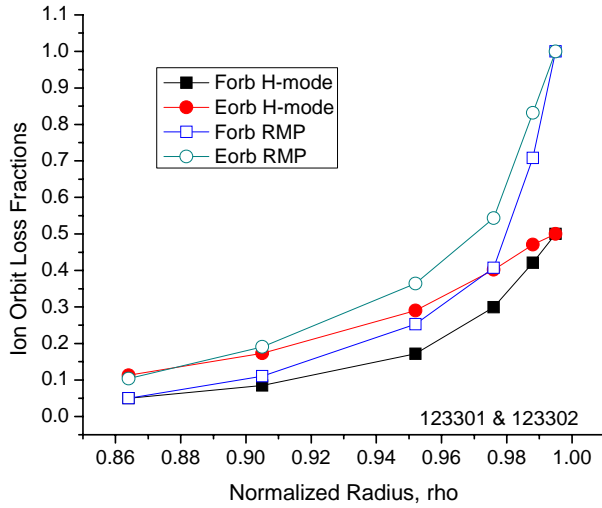
Figure 14 Ion particle and energy cumulative loss fractions for ion orbit loss in DIII-D RMP and otherwise similar H-Mode discharges.
