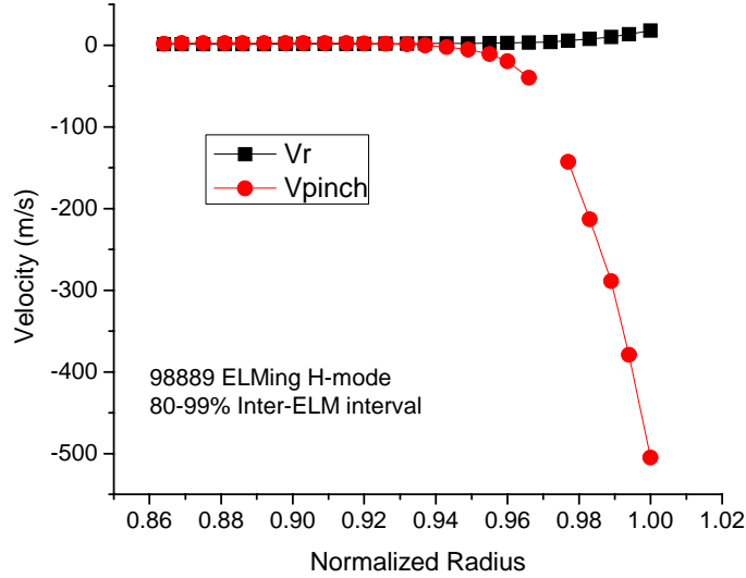
Figure 6 Comparison of the importance of recycling neutrals ( V_r ) and V_{xB} and E_{rad} ( V_{pinch} ) in determining the pressure gradient in the edge pedestal.
